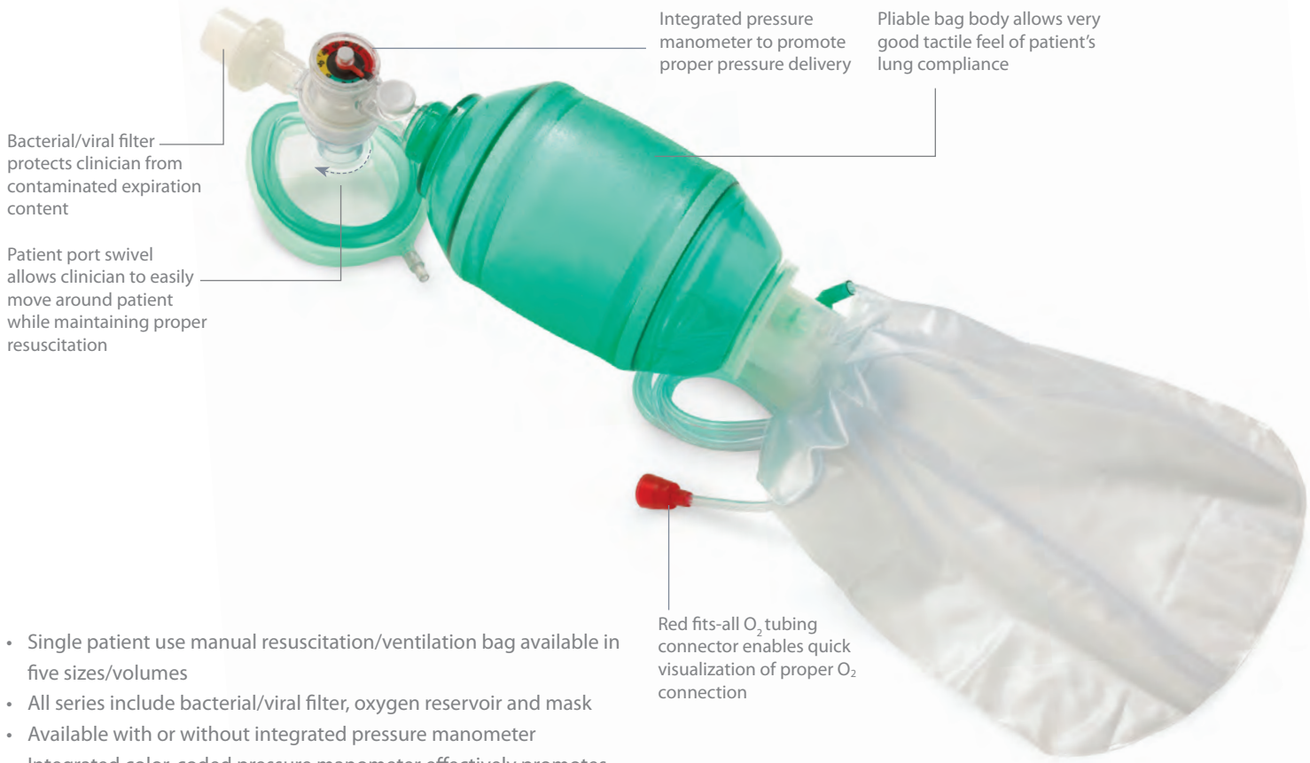
Adult AirFlow AF1140-Series Shown with B/V filter, integrated pressure manometer and inflatable adult mask
